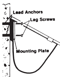
Figure 2. Concrete Walls
