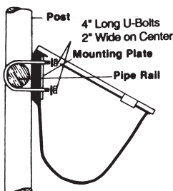
Figure 3. Pipe Corral
