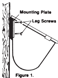
Figure 1. Wood Walls
